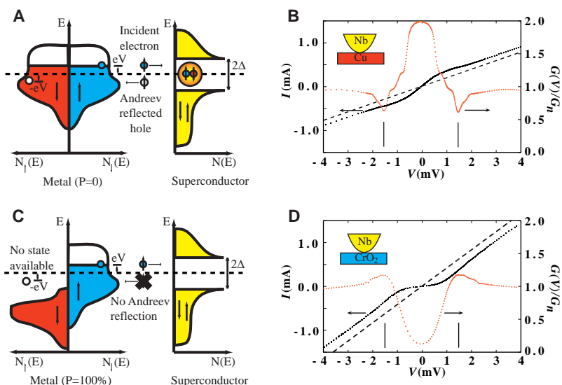
Fig. 1. Supercurrent conversion at the superconductor-metal interface for spin polarizations of P = 0 and P \rightarrow 100\% . (A) Schematic of the process for P = 0 when the Andreev reflection is unhindered by a spin minority population at E_F . The solid circles denote electrons and open circles denote holes. (B) Experimental measurement of the I - V and differential conductance dI/dV at T = 1.6 K via a superconducting Nb point contact on Cu. The vertical lines denote the bulk gap of Nb: \Delta(T = 0) = 1.5 meV. The dashed line is the normal state I - V for a conductance of G_n = 0.194 ohm ^{-1} . (C) Schematic of process for P \rightarrow 100\% when there is no supercurrent conversion at the interface. (D) Experimental I - V and dI/dV at T = 1.6 K via the Nb point contact on \text{CrO}_2 . The dashed line is the normal state I - V for a conductance of G_n = 0.417 ohm ^{-1} .
